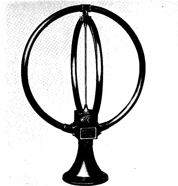
D.F. Loop Aerial Type 354NA/52 (Short Pedestal)
