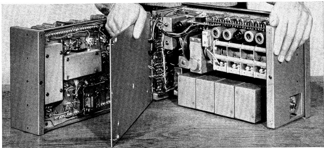
The receiver opened up showing how the book-like construction renders all components readily accessible.
