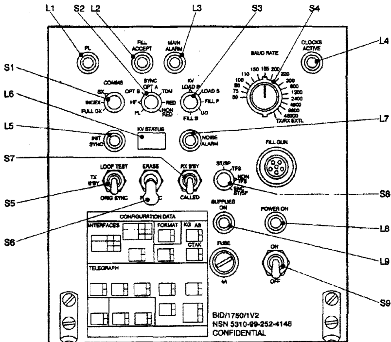
Figure 1. BID/1750/1V2 Front Panel
