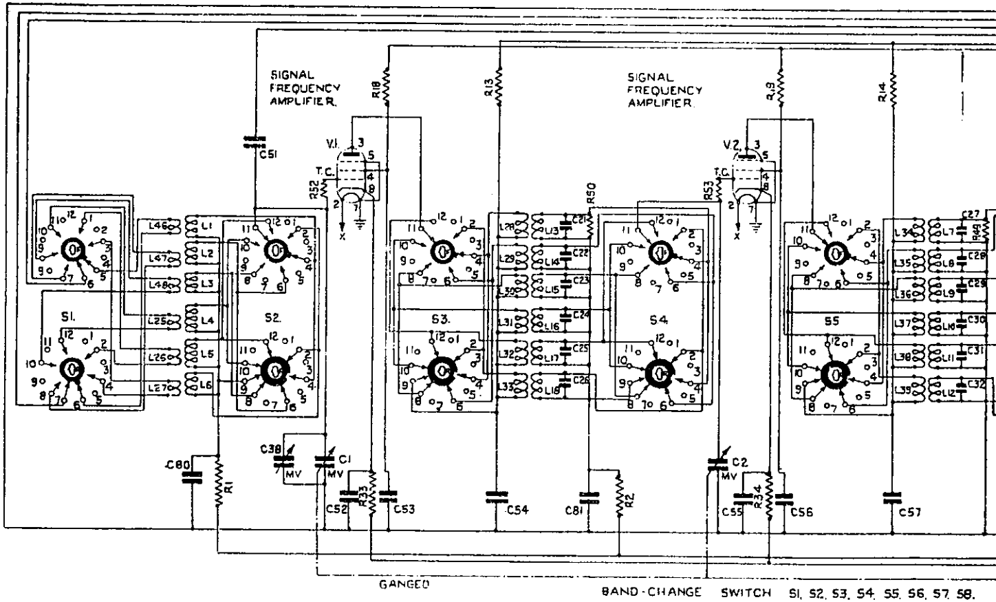
Complete circuit diagram of the CR100
