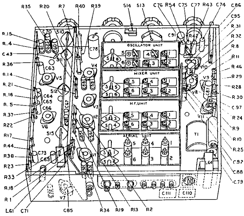
Top and underside layouts of the CR100
