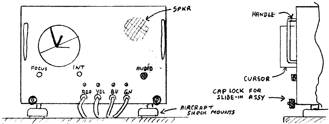
UPD 501 BLOCK DIAGRAM & PICTORIAL SKETCH (1952 - 53)
