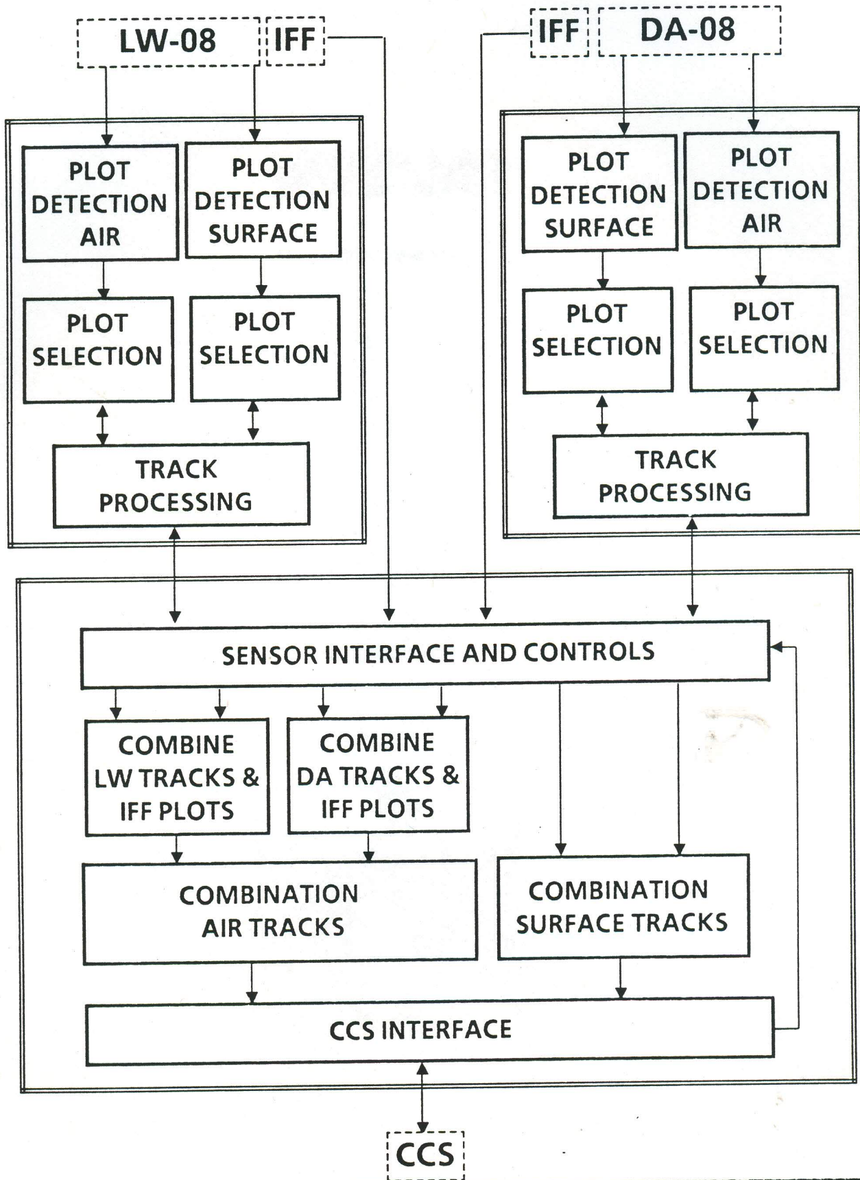
ATMS FUNCTIONAL BLOCK DIAGRAM
