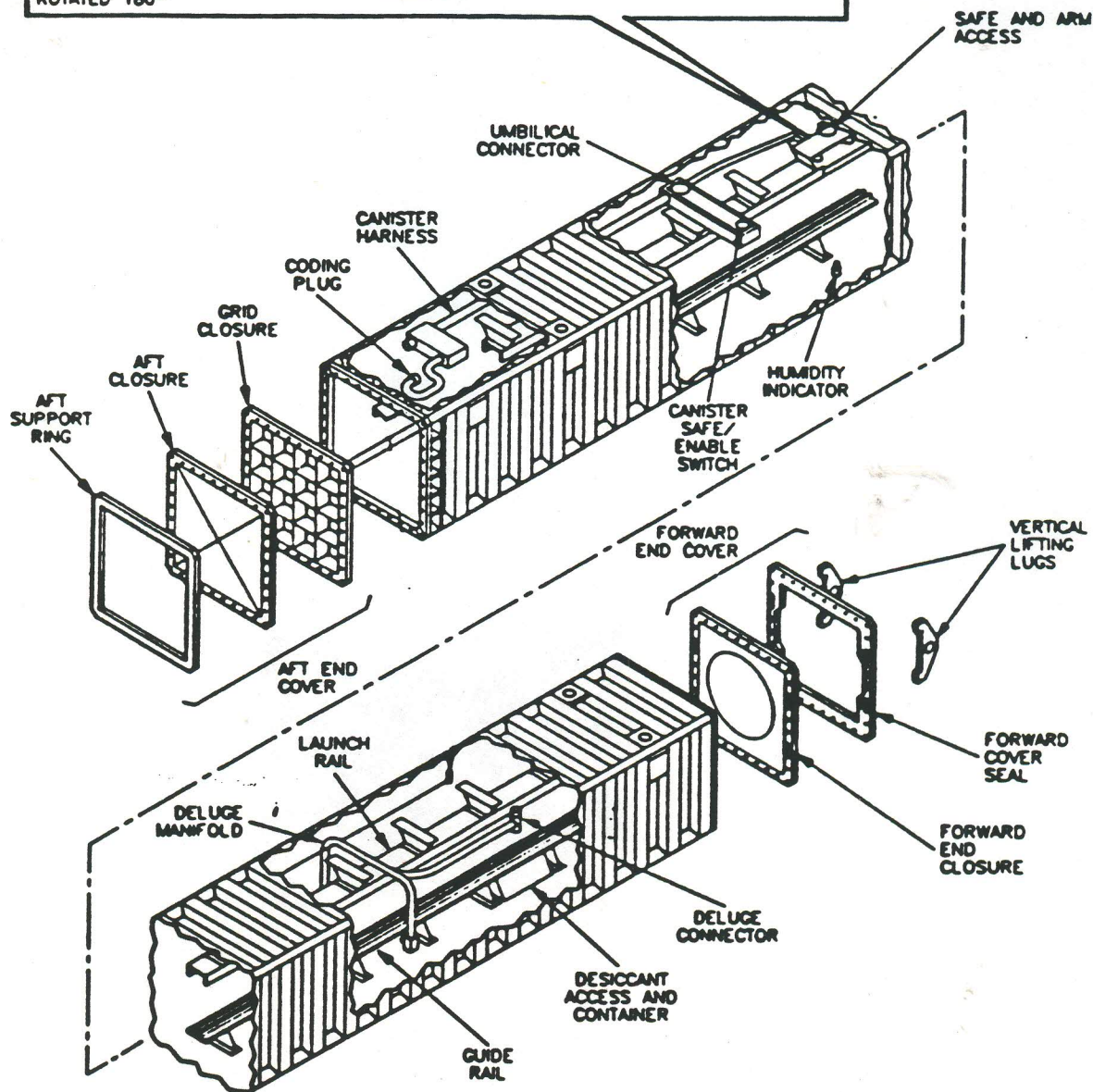
MK 13 MOD 0 CANISTER
