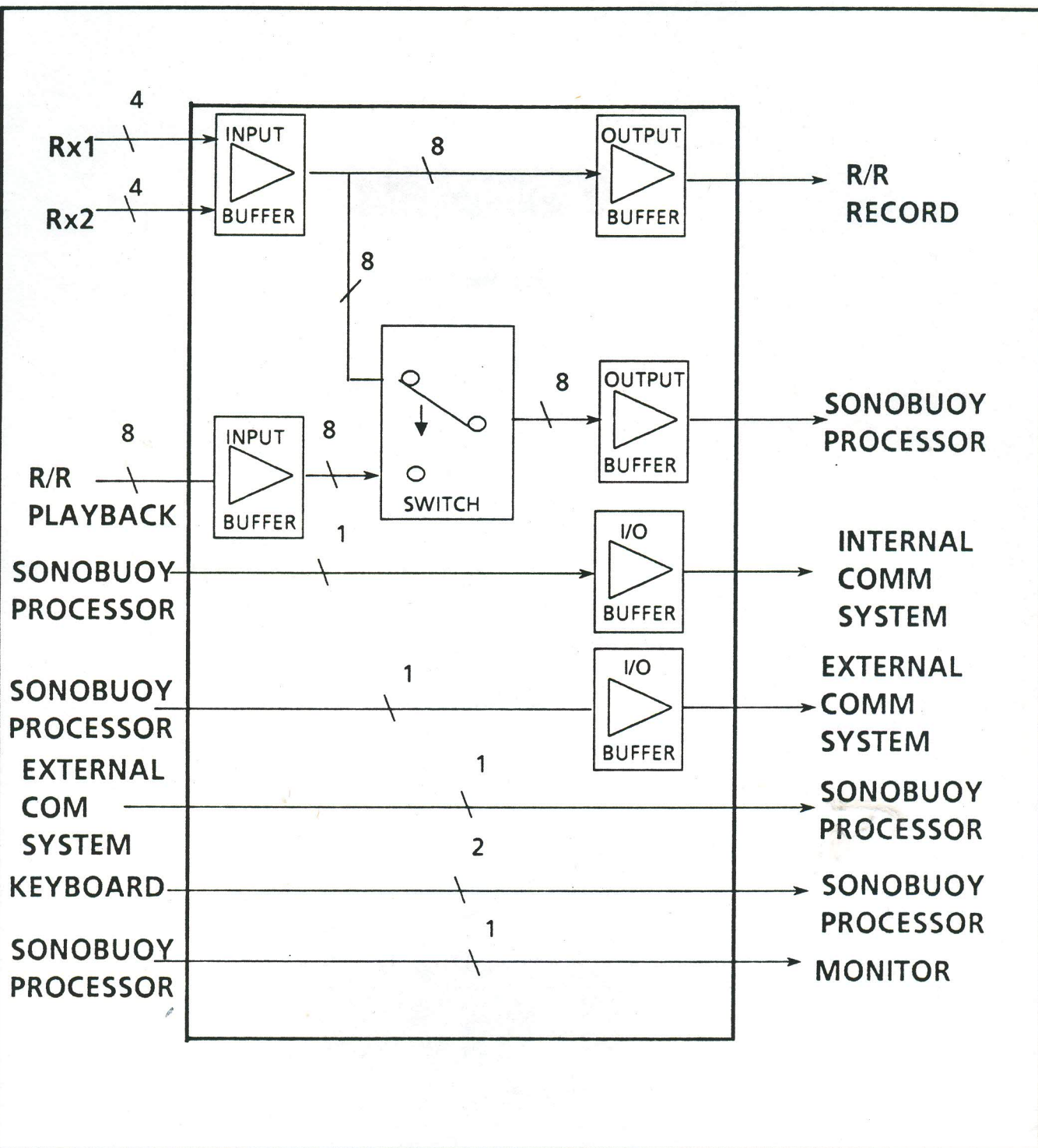
AUDIO CONTROL BOX
