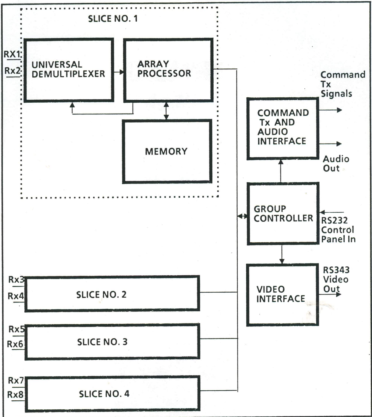
SONOBUOY PROCESSOR
