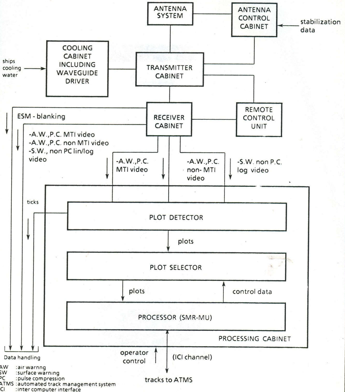
Figure 6 LW08 Long Range Radar Functional Block Diagram
