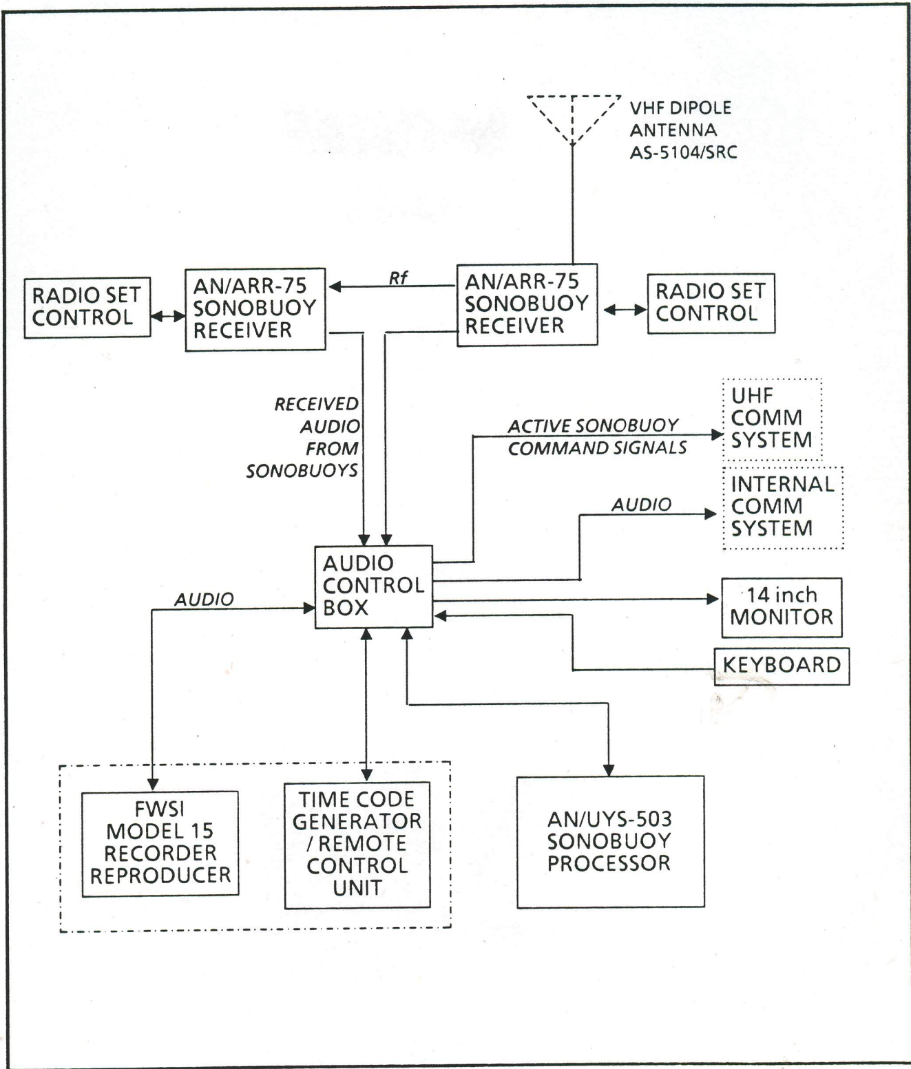
Figure 22 Sonobuoy Processing System
